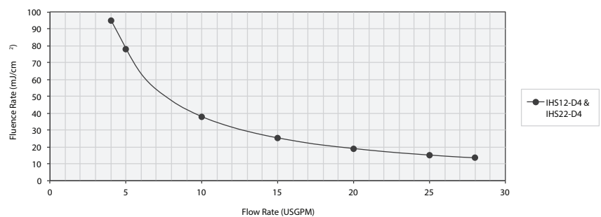
IHS12-D4 & IHS22-D4 DOSE CURVES
